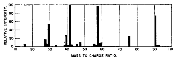
Fig. 5.—Mass spectra of 2-methyl-2-propanethiol.
