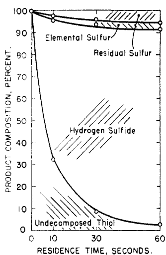
Fig. 4.—Effect of residence time on sulfur distribution at 450°.
